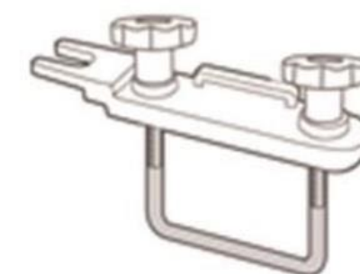
U型螺杆固定 U-Shaped Screw Fixing
